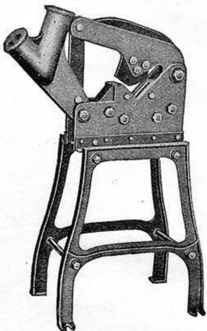
Buffalo Angle Cutter No. 2
