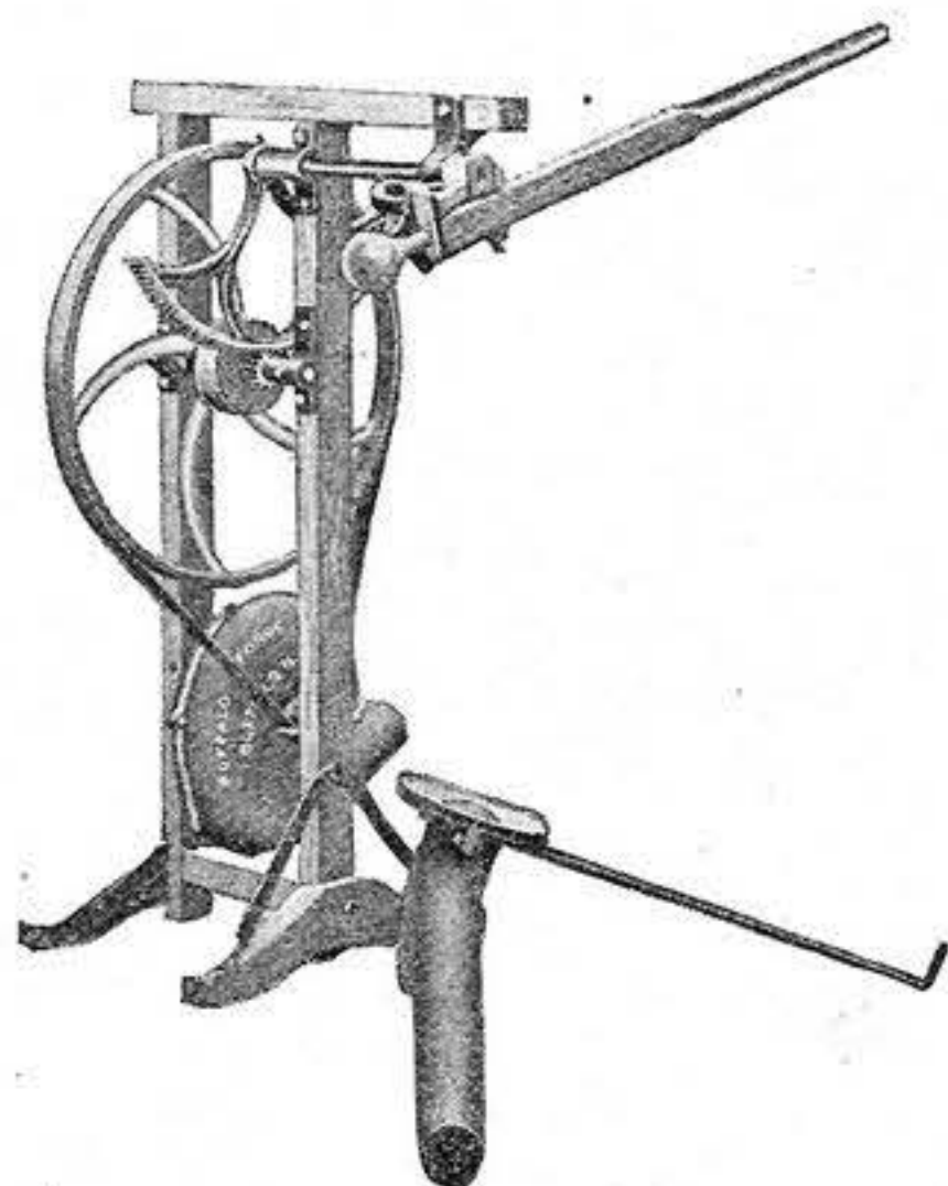
No. 3 Hand Blower Price $25.00 Fan 14 Inches. Weight 130 Lbs.
