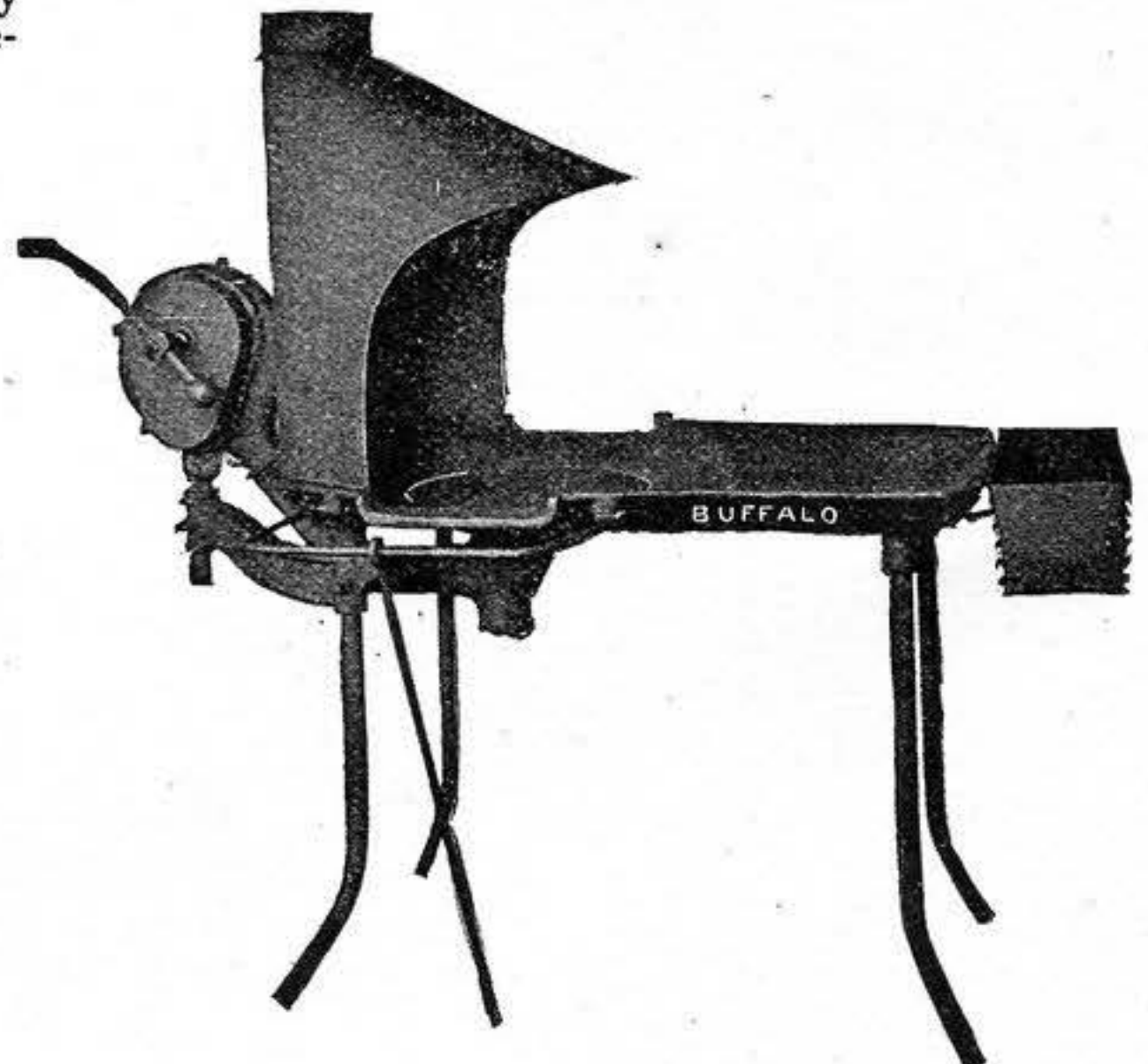
No. 124. Blacksmiths' Forge
