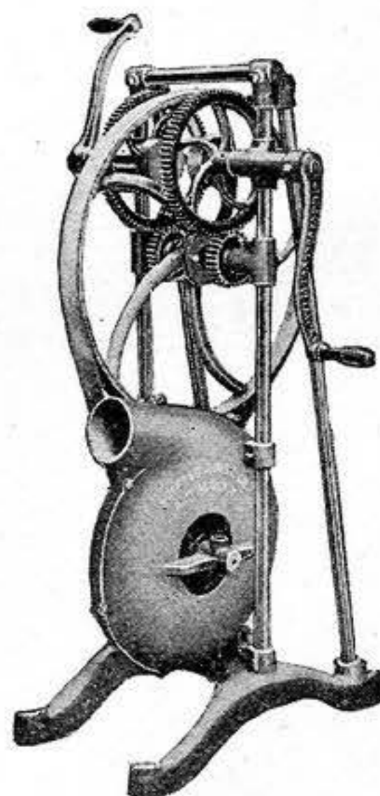
No. 7 Double Crank Hand Blower Price $32.00 Fan 17 Inches. Weight 195 Lbs.
